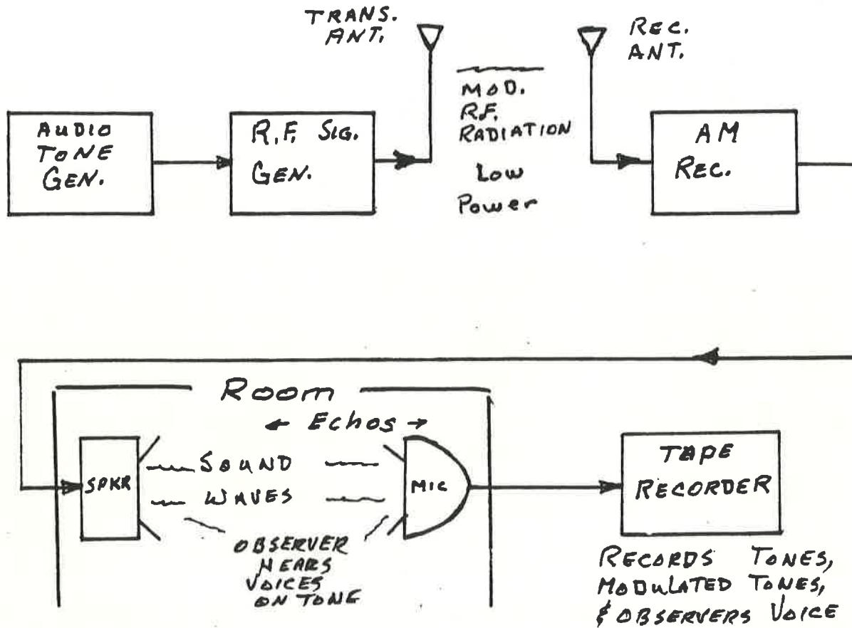
Fig. 11 Functional Block Diagram of Mark IV
